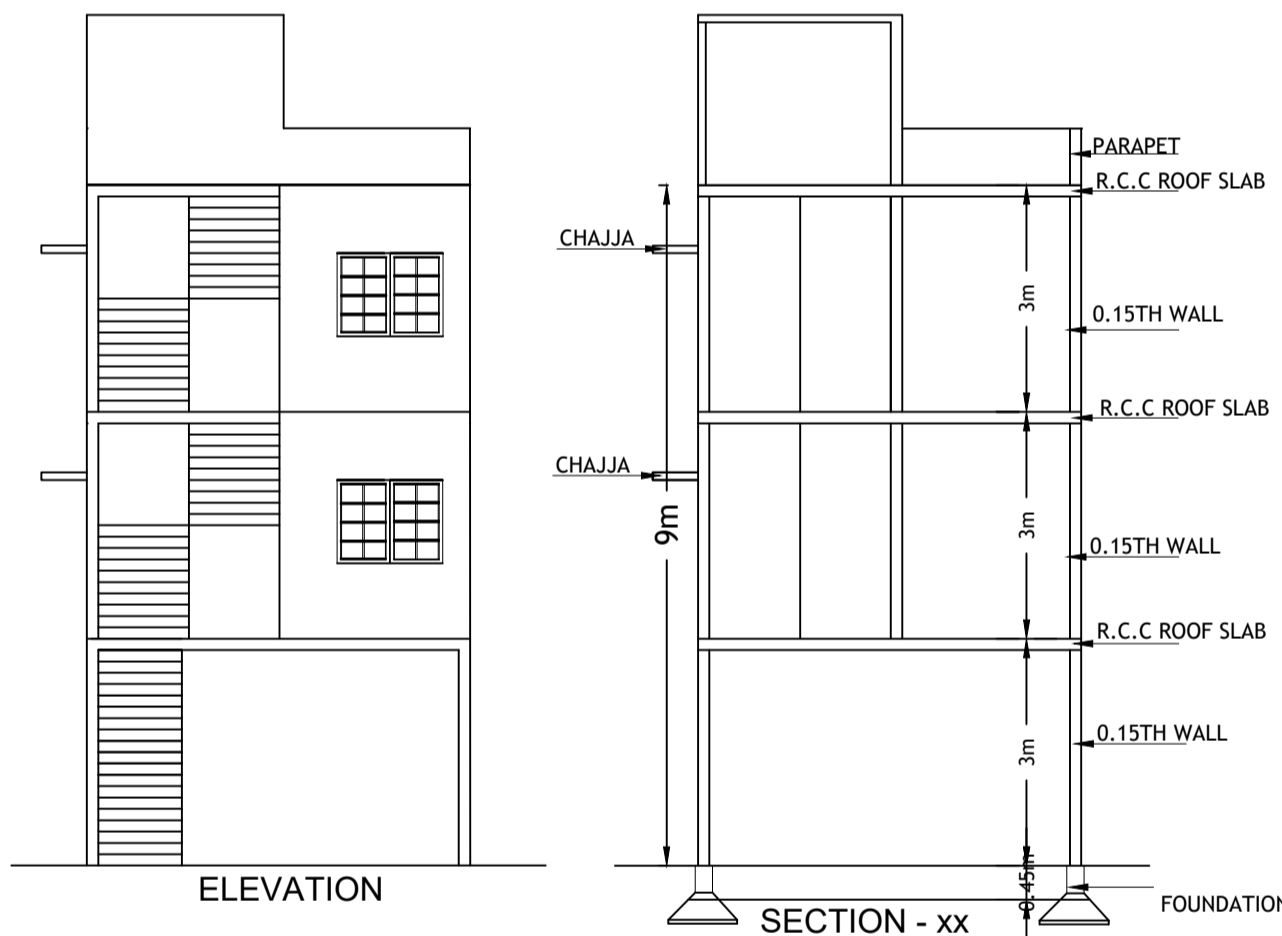
SECTION - xx
